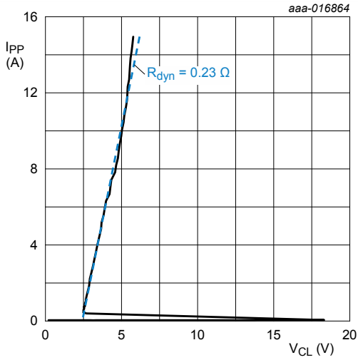
Fig. 7. Dynamic resistance with positive clamping voltage
