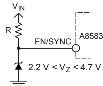
Figure 4. Automatically enabling the A8583 from VIN or some other power rail
